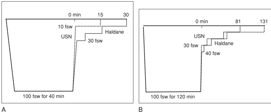
Figure 4-8. A. A decompression schedule from Haldane's first table 5 . Schedules from this table have deeper first stops and more decompression time than corresponding U.S. Navy schedule 9 . B. A decompression schedule from Haldane's second table. Schedules from this table have deeper first stops but less decompression than corresponding U.S. Navy schedules.
