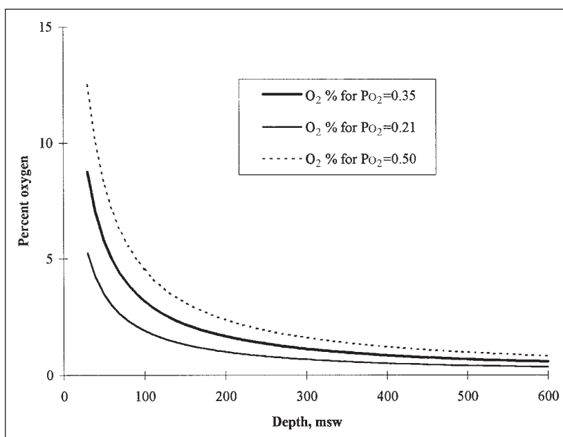
Figure 6-4. Range of oxygen concentrations for deep saturation diving. The heavy solid line represents the oxygen concentration needed to maintain 0.35 atm, a common choice for P_{O_2} . The lower line represents the oxygen concentration needed to maintain the normoxic level of 0.21 atm. The dotted line represents the upper limit of continuous exposure to avoid whole-body toxicity, 0.5 atm. The low oxygen concentrations needed are difficult to mix and analyze within acceptable tolerance limits, and they are therefore usually mixed as the chamber is being pressurized.
