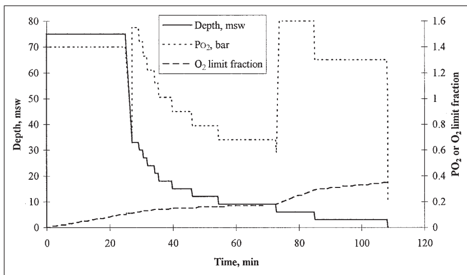
Figure 6-9. Profile of a technical trimix bounce dive to 75 msw for 25 min. This profile has been used many times without incident (the profile depicted is for display only and should not be used because it lacks some minor conservative modifications). The gas is switched to a 36% oxygen-enriched air mixture at the first stop at 33 msw and to pure oxygen at 6 msw. The upper dotted line shows the PO_2 , and the lower dashed line shows the buildup of the “oxygen limit fraction” (or CNS % ), which reaches 0.35. Compare this profile with that in Figure 6-10.
