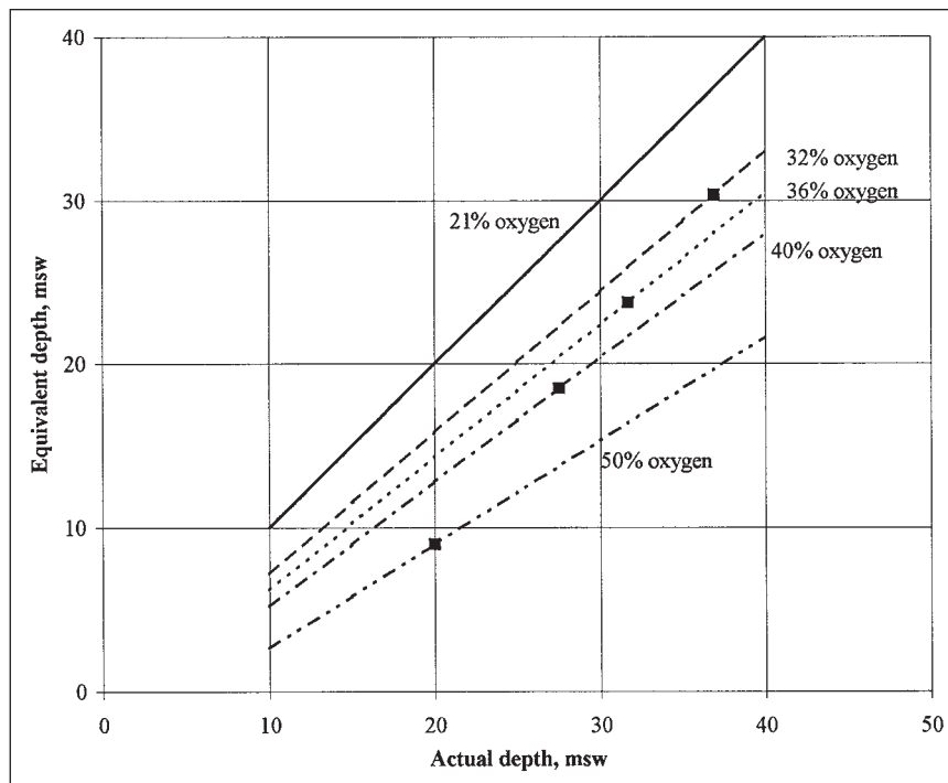
Figure 6–8. “Equivalent air depths” for decompression with enriched air mixtures. The curves show the depth of a dive with air that has the same \text{PN}_2 as the actual depth indicated. A decompression table for the equivalent depth can be used. The square markers indicate the point at which the \text{PO}_2 reaches 1.5 atm, a reasonable oxygen tolerance limit. Each gas should be used only for the range to the left of the marker; for example, with 50% oxygen, only dives at an actual depth of 20 msw or shallower should be done.
