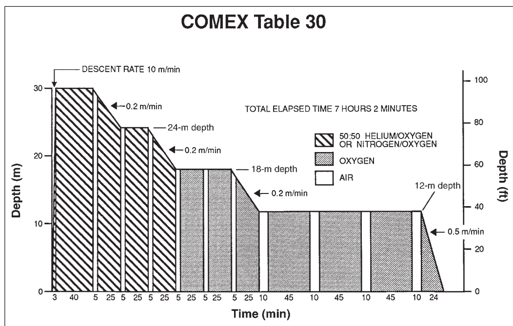
Figure 10-8. Stolt Offshore (Formerly Comex) Table 30. This table is an option for treating serious decompression illness, with a maximum pressure of 4 ata (30 m). Some anecdotal evidence suggests that He-O 2 may be more efficacious than other breathing gases, and this table allows the option of using heliox when the pressure is greater than 2.8 ata. (From Moon RE, Gorman DF: Treatment of the decompression disorders. In Bennett PB, Elliott DH [eds]: The Physiology and Medicine of Diving. Philadelphia, WB Saunders, 1993, pp 506-541.)
