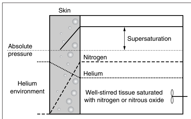
Figure 7-12. A model of inert gas exchange during isobaric cutaneous counterdiffusion based on the Hills model 15 in which well-stirred tissue is separated from the environment by a diffusion barrier. A rapidly diffusing gas (helium) surrounds the body while the inspired gas (nitrogen) is slowly diffusing. Helium diffuses into the body through the skin faster than nitrogen diffuses out, resulting in supersaturation and bubble formation in the diffusion barrier. As the bubbles grow, they cause the tissue damage shown in Figure 7-11.
